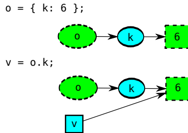
Figure 3: Trivial Property Read
