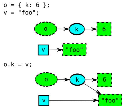
Figure 2: Property Write without Strong Update
