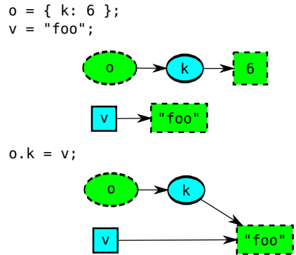
Figure 1: Property Write with Strong Update
