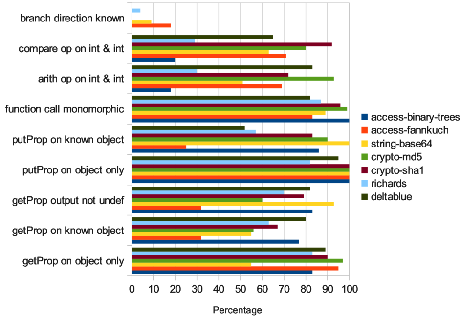
Figure 5: Analysis Accuracy Statistics
