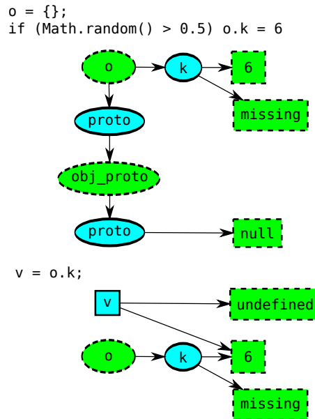
Figure 4: Property Read on Potentially Missing Property
